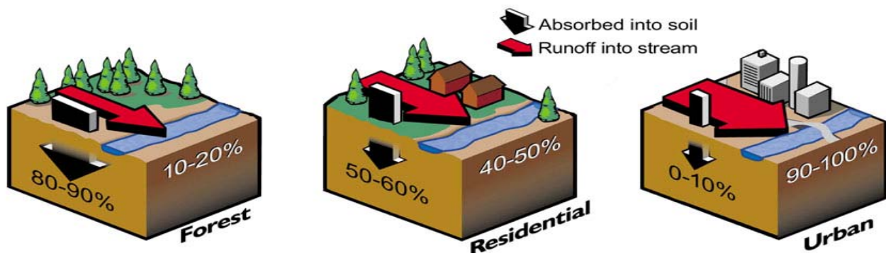
Figure 1.1-2 Changes in Hydrology and Runoff Due to Development Based on Marsh, 1983. Graphic courtesy of Atlanta Journal-Constitution
